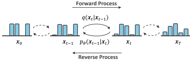
Figure 2: An overview of DiffRec, where the histogram denotes the corrupted interactions of a user over all items. The forward process gradually corrupts the user’s interaction history by the transition step q(x_t|x_{t-1}) , and then the model learns to recover x_0 using p_\theta(x_{t-1}|x_t) step by step.
